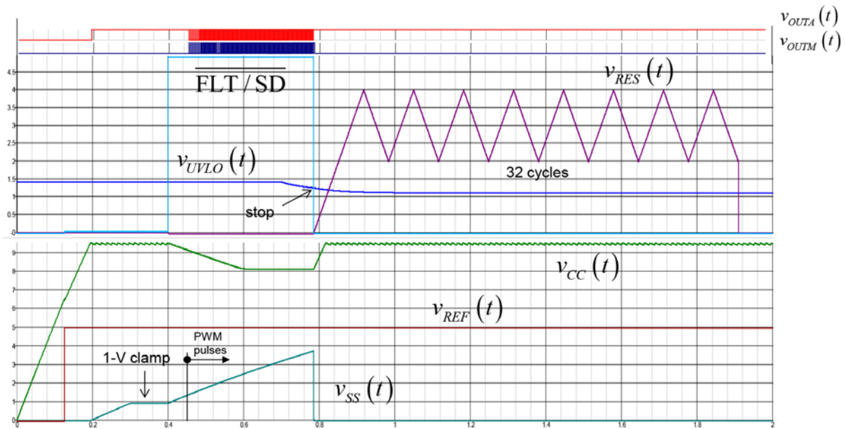
Figure 50. The Input Voltage is Going Down and Puts the Part in Standby Mode. It cannot restart prior to cycling the RES capacitor 32 times
