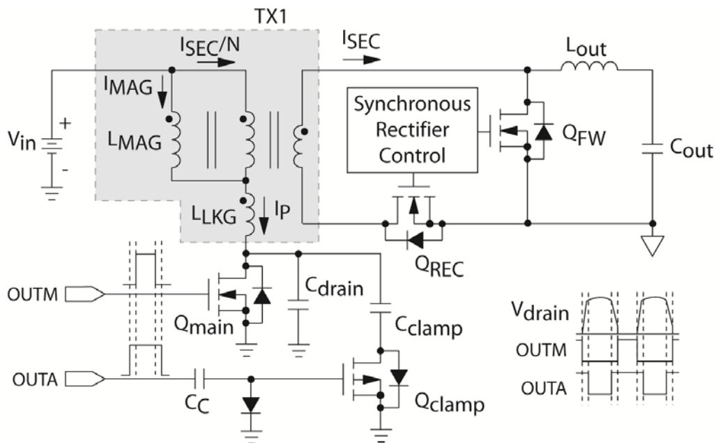
Figure 60. Active-clamp Forward Topology
