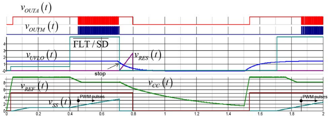
Figure 51. The Part Starts up while V_{in} is ok. V_{in} now decreases to 0, shutting off the part. V_{in} is back again shortly after, restarting the part.
