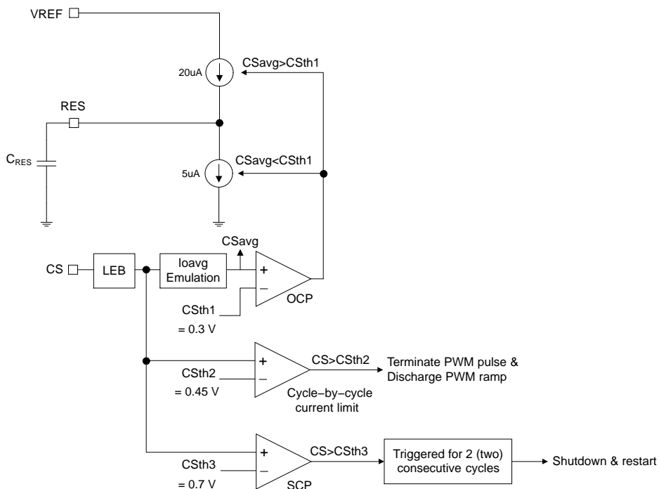
Figure 52. The Current Limit Circuitry Implements Three Distinct Comparators
