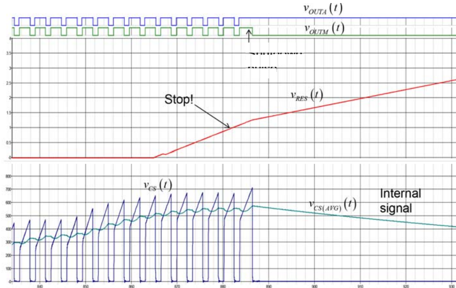
Figure 58. Overload Condition Operating Waveforms
