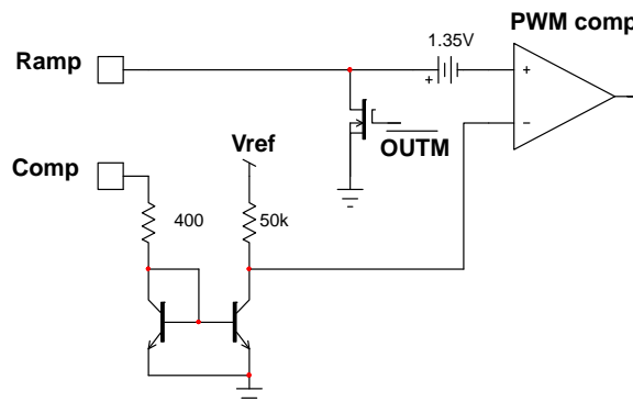
Figure 56. COMP Input Architecture
