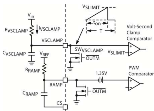
Figure 55. The VSCLAMP Configuration in Peak Current-mode Control
