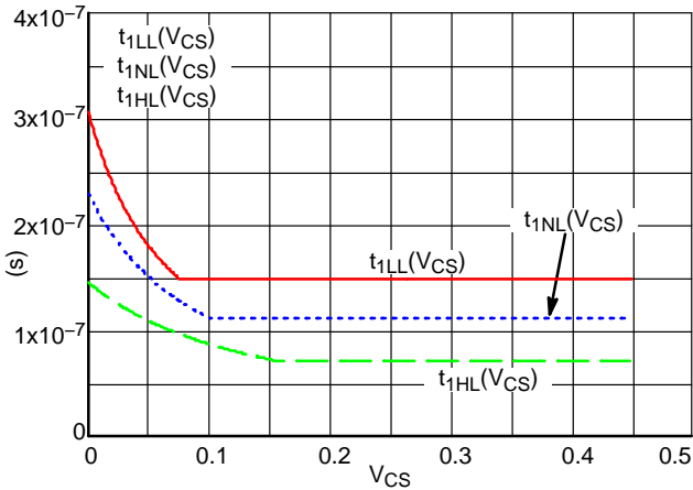
Figure 62. The Dead Time Evolution with Input Voltage and the Sensed Current
