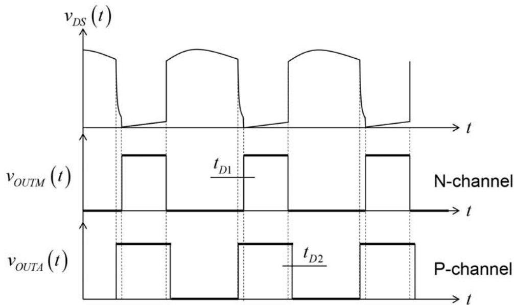
Figure 61. Overlap Time Waveforms
