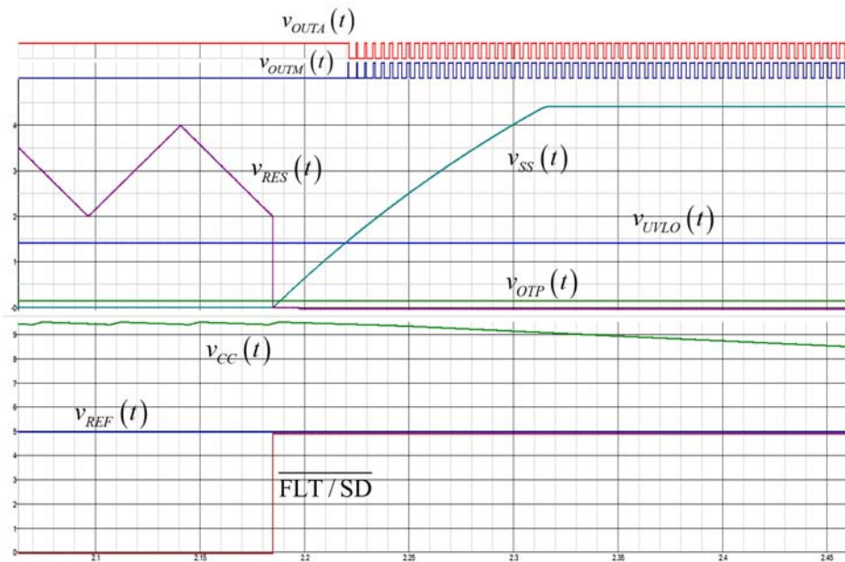
Figure 59. Timing Diagram Exiting Restart
